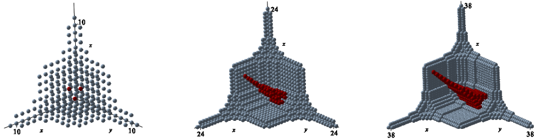
Figure 5.1: \mathfrak{X}_r^{\mathcal{B}_2} , for r \in \{6, 13, 20\} : the points in purple do not belong to \mathcal{C}_r^2 + \mathcal{C}_r^2 + \mathcal{C}_r^2 . In other words, the represented lattice points index the necessary nodes of evaluation for the sparse interpolation of any sum of r monomial (grey) or r Chebyshev polynomials associated with \mathcal{B}_2 (grey and purple).
