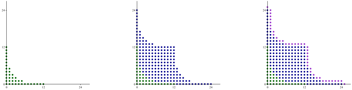
Figure 3.1: \mathcal{C}_{13}^2 , \mathcal{C}_{13}^2 + \mathcal{C}_{13}^2 and \mathcal{C}_{13}^2 + \mathcal{C}_{13}^2 + \mathcal{C}_{13}^2 .
