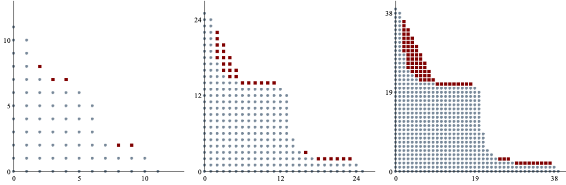
Figure 5.1: \mathfrak{X}_r^{\mathcal{B}_2} , for r \in \{6, 13, 20\} : the points in purple do not belong to \mathcal{C}_r^2 + \mathcal{C}_r^2 + \mathcal{C}_r^2 . In other words, the represented lattice points index the necessary nodes of evaluation for the sparse interpolation of any sum of r monomial (grey) or r Chebyshev polynomials associated with \mathcal{B}_2 (grey and purple).
